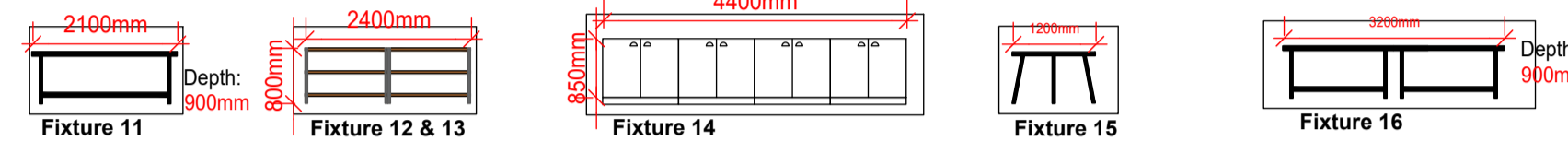
Display Furniture Scale 1:100@A1 / 1:200@A3
